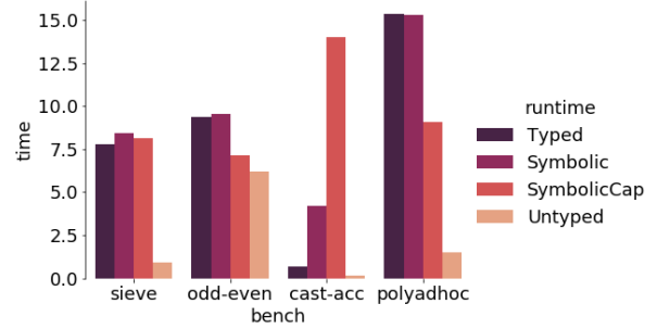
Fig. 7: Full Benchmarks
