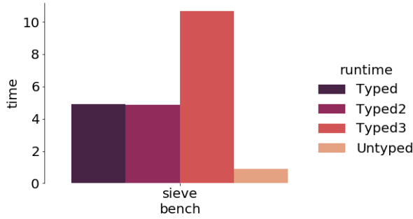
Fig. 6: Sieve Benchmark
